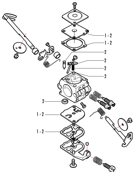
FIGURE 3 - WALBRO WT 170
